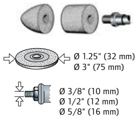
Type 16, 17, 18, 18R, and 19 Cone and Plug Wheels
