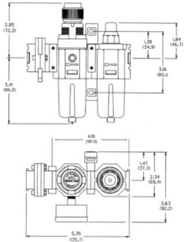
Dimensional Data Dimensions – in (mm)
